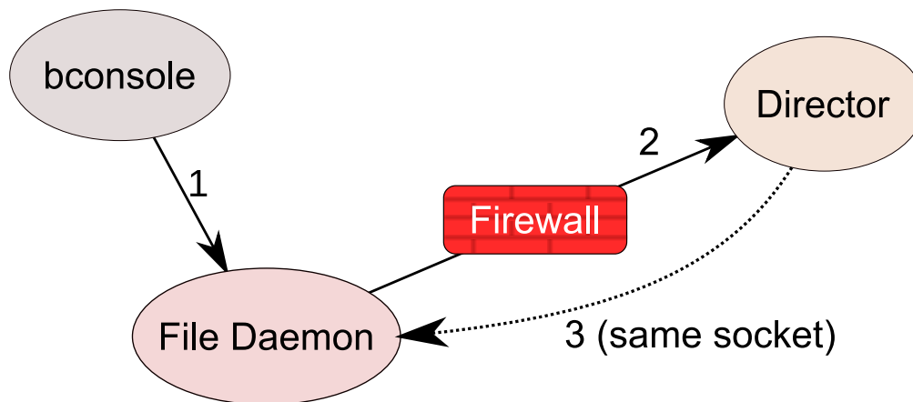
Figure 6.2: Client Initiated Backup Network Flow
