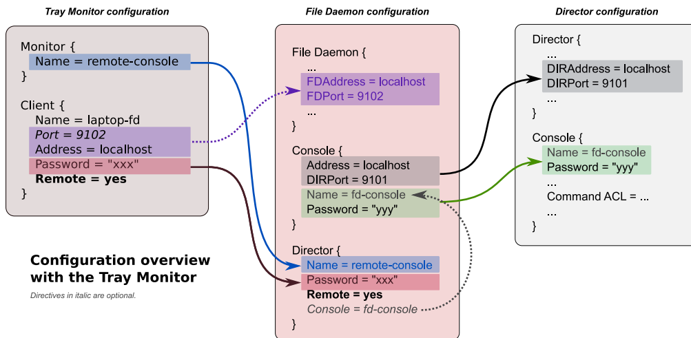
Figure 6.4: Relation Between Resources (tray-monitor)
