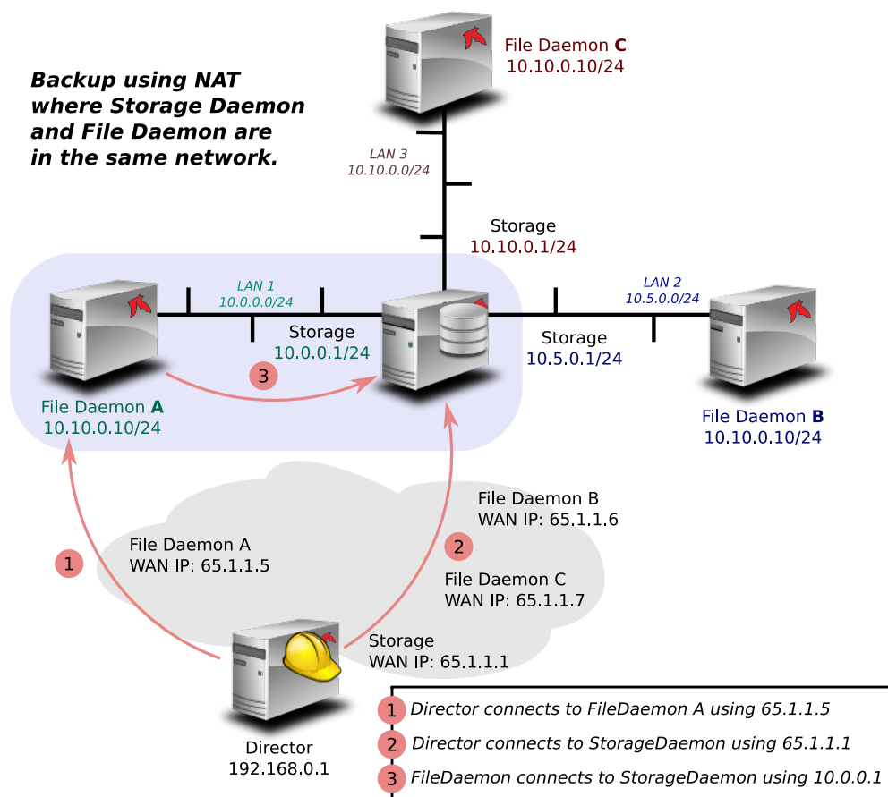
Figure 21.3: Backup over WAN using FD Storage Address
