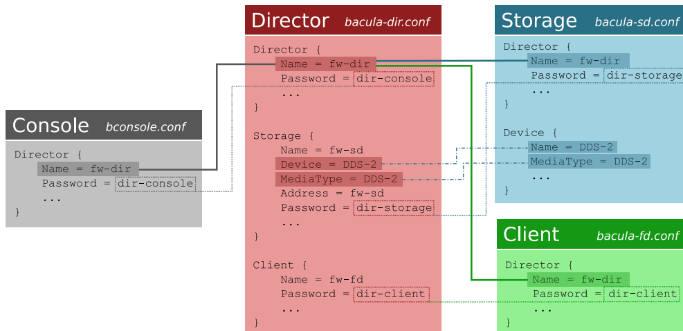
Figure 20.2: Configuration diagram
